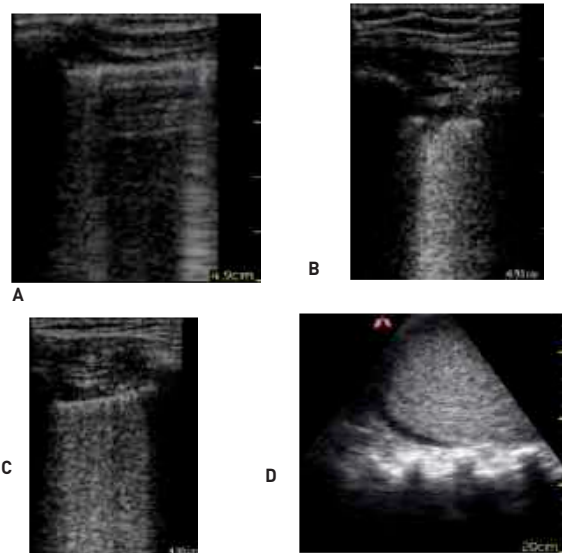
Figure 1: a) Linear view LUS, with skip B-line profiling and preserved A-line profiling in early COVID-19 pneumonitis; b) Confluent B-line profiling, sub-pleural consolidation and irregular thickened pleura in medium severity COVID-19 pneumonitis; c) Confluent B-line profiling and obliteration of all A-lines in severe COVID-19 pneumonitis; d) Basal consolidation, parapneumonic effusion and spine sign seen at the base of a COVID-19 patient with severe pneumonitis.
