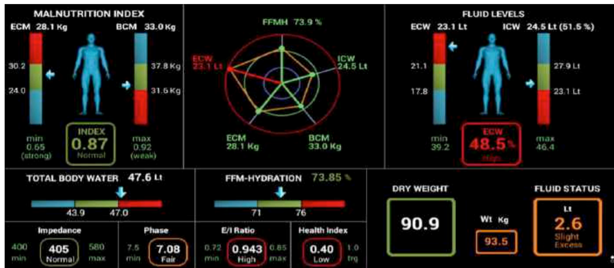
Figure 1. Sample screenshot with results obtained via full body, multifrequency bioelectrical impedance analysis (BIA) with touch i8 device (Maltron, UK) showing a volume excess of 2.6 litres and an increased ECW:ICW ratio of 0.943 indicating capillary leak. The patient’s fluid composition is monitored with BIA separating intra- and extracellular water and estimating the volume excess [Source: Myatchin et al. 2020].
